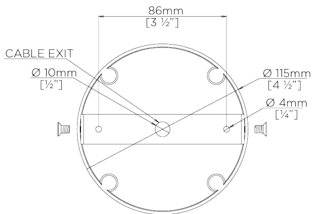
CEILING MOUNT BRACKET
