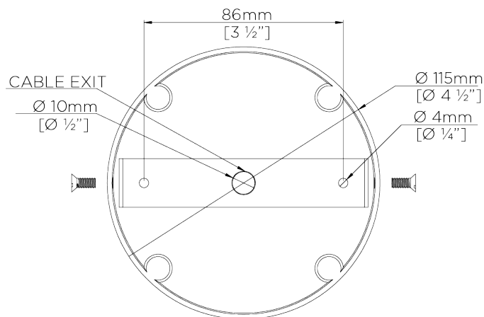
CEILING MOUNT BRACKET
