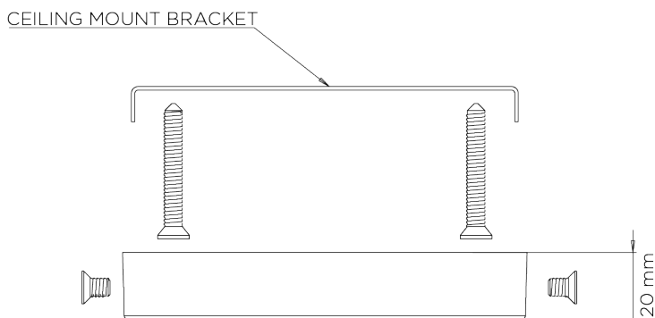
CEILING ROSE DETAIL
